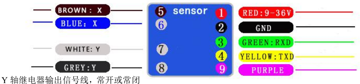
LVT553T 接线图
